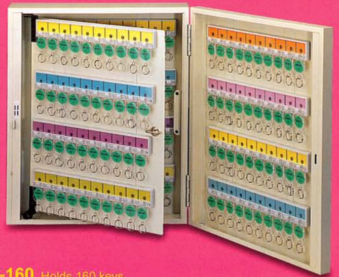
K-160 Holds 160 keys. Size: 500H X 420W X 110 D m/m Weight: 12.7 Kg Color: beige
